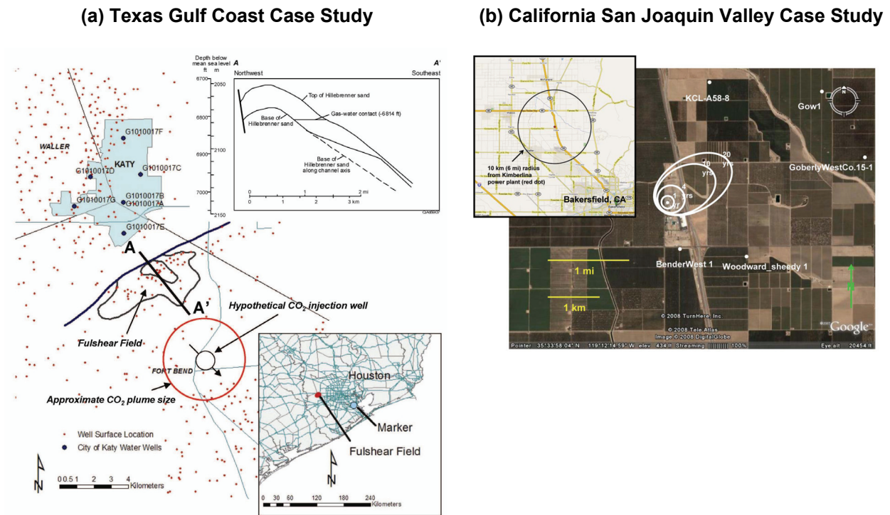
Figure 3. (a) Location map of a hypothetical GCS project in the Texas Gulf Coast showing oil and gas wells (small red dots), water wells, Fulshear gas reservoir, and injection well in the water leg of the Hillebrenner Sand. Upper inset shows cross section through the Fulshear gas reservoir showing growth fault, gas cap, and down-dip water leg. Note vertical exaggeration; dip of the Hillebrenner is approximately 1° to the southeast. (b) Location of the Kimberlina site with prediction of footprint of the CO 2 plume from TOUGH2 numerical model along with nearby wildcat wells.
